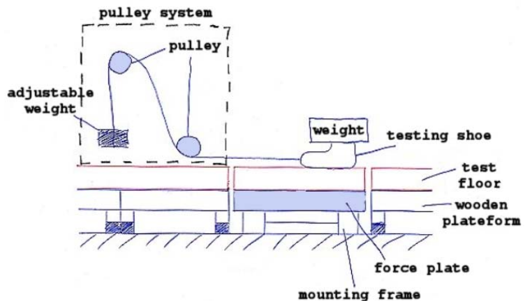
Figure 1 – mechanical slip resistance test setup
